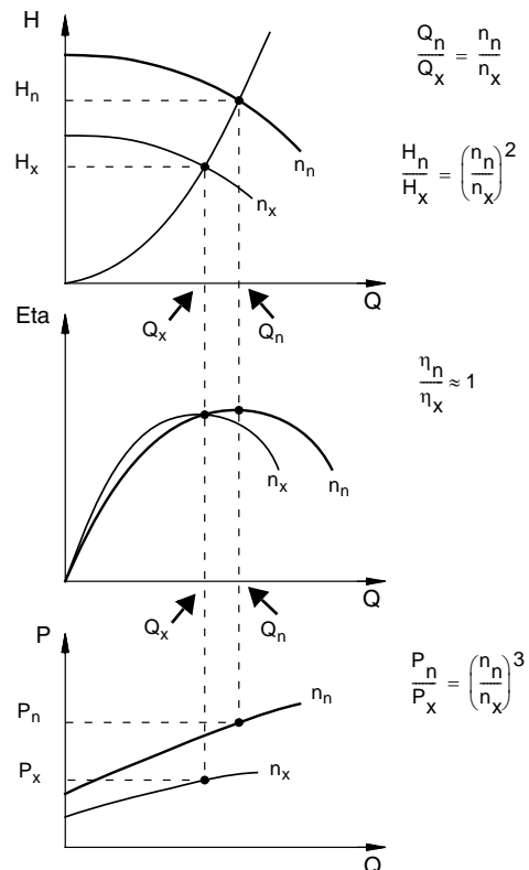
Fig. 22 Affinity equations
